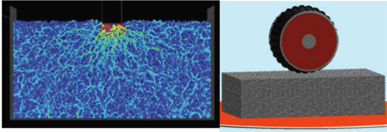
Figure 16: (Left) Rigid punch penetrating a box of particles, simulated using DEM. Highly stresses load paths, termed load chains, emanate from the area of surface contact [26]. (Right) Case study: Mars exploration rover wheel digging simulation using DEM. Particles and material properties were scaled up in order to minimize computational cost [27].
