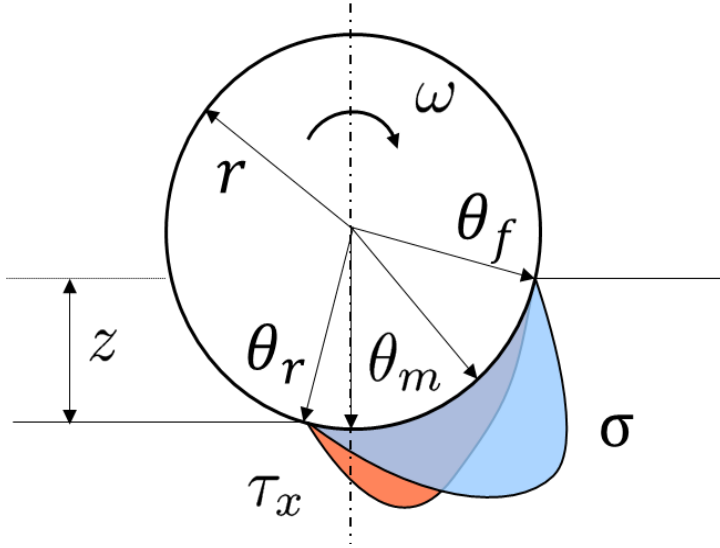
Figure 7: Schematic representation of normal and tangential stress profile along a rigid wheel.
