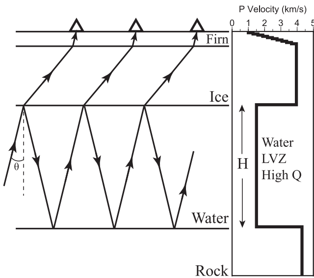
Figure 5. Illustration of how trapped waves in the slow water layer propagate to the free surface. The 1-D P -wave velocity model is plotted to the right as reference. See the text for more details.
