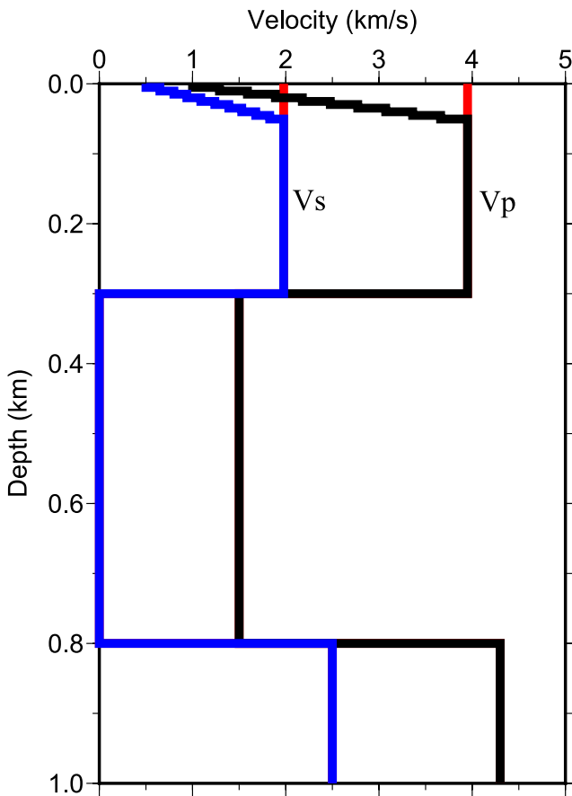
Figure 2. The 1-D P - and S -wave velocity models used to compute synthetic Green's functions. Differences between the two 1-D models with or without the top 50-m firn layer are highlighted by the red segments.
